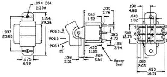
3PDT Part No.R301R1A1QE
