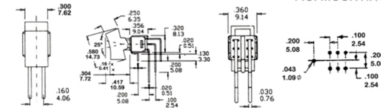
DPDT Part No. RS-51RS5A4QN
