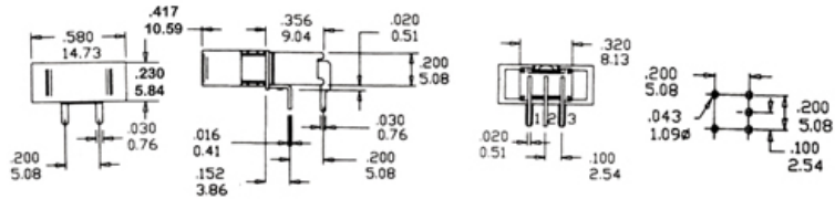
SPDT Part No. RS-41RS4A3QN
