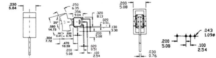
SPDT Part No. RS-41RS5A4QN
