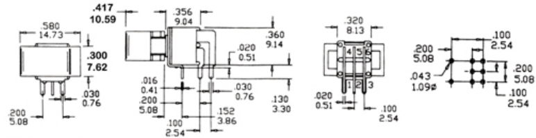
DPDT Part No. RS-51RS5A3QN
